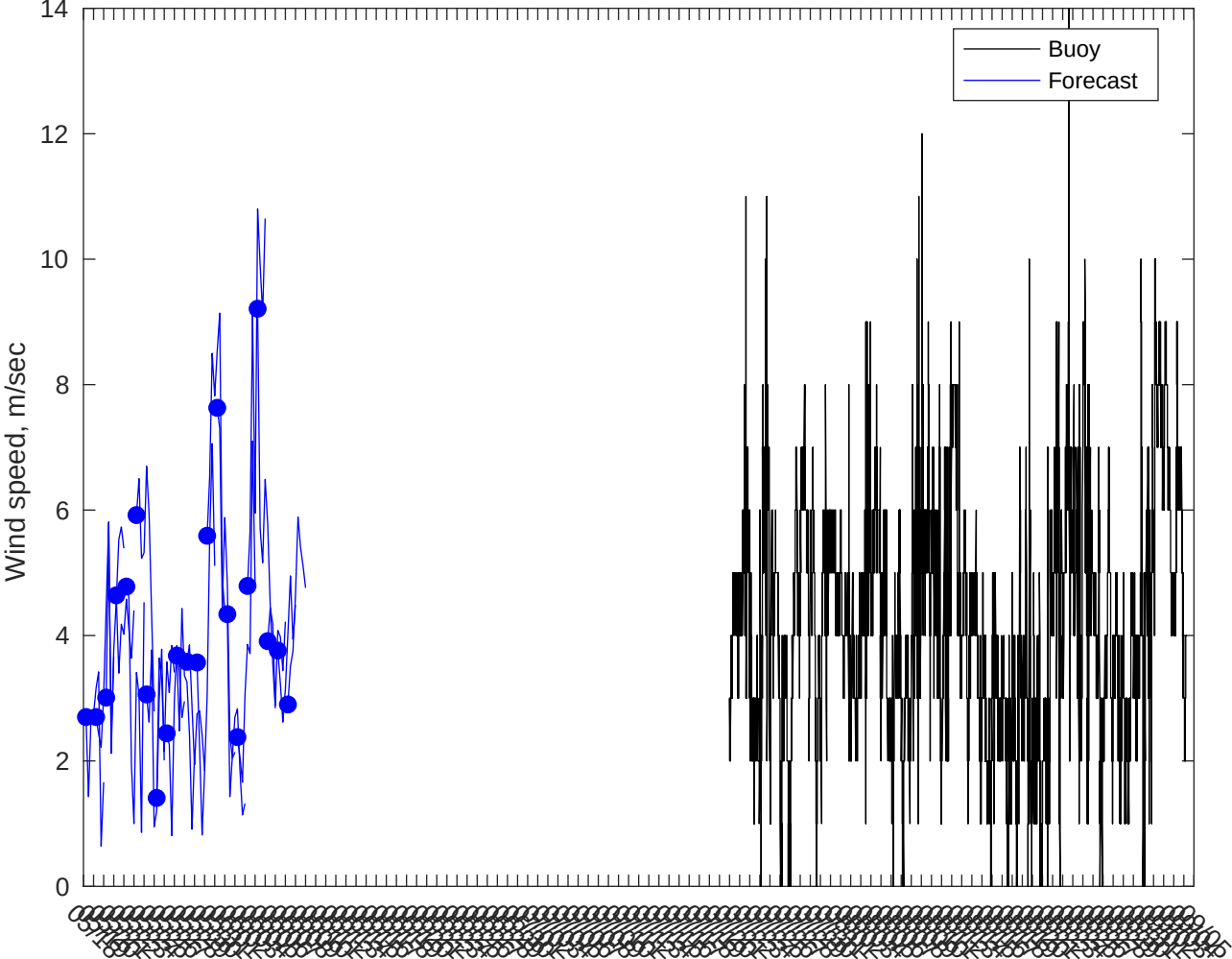
NDBC 42036 vs AUSWAV Winds: 3 to 5 day forecast
