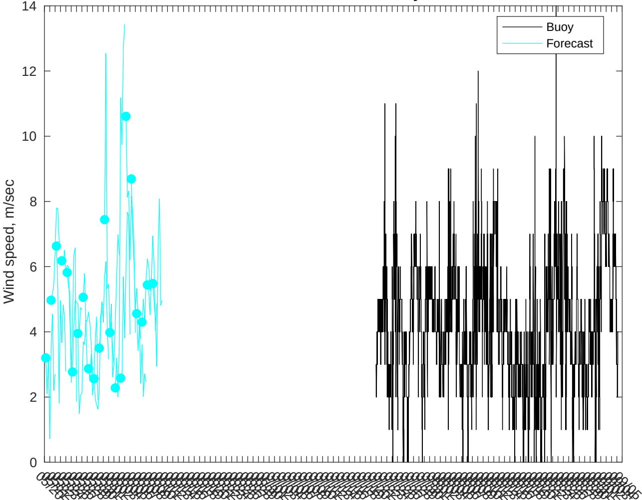
NDBC 42036 vs AUSWAV Winds: 5 to 7 day forecast
