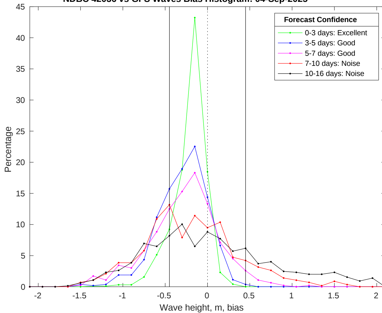
NDBC 42036 vs GFS Waves Bias Histogram: 04-Sep-2025
