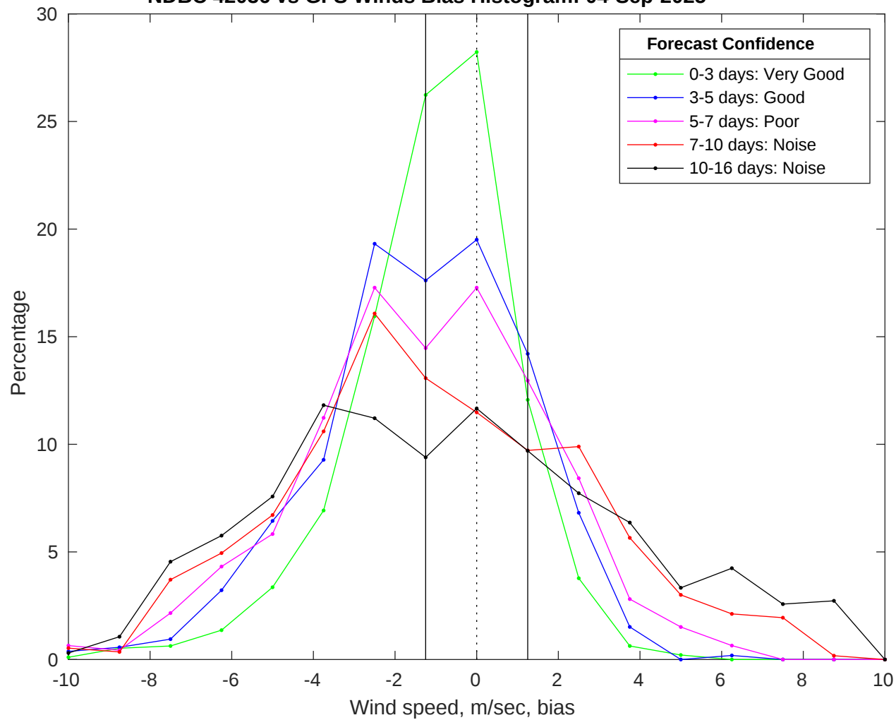
NDBC 42036 vs GFS Winds Bias Histogram: 04-Sep-2025
