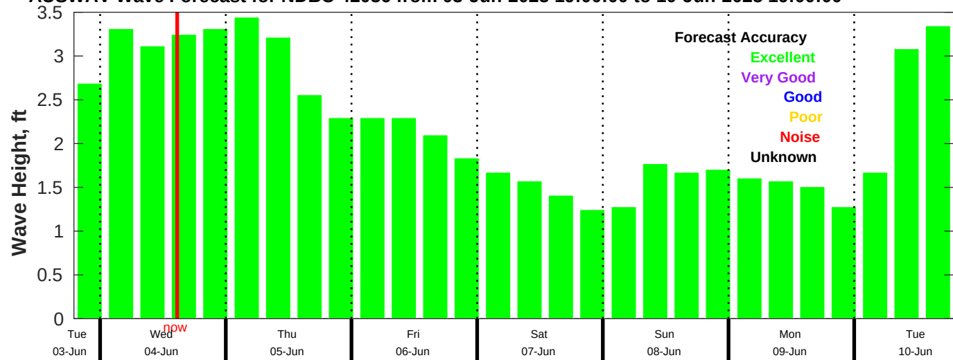
AUSWAV Wave Forecast for NDBC 42036 from 03-Jun-2025 19:00:00 to 10-Jun-2025 19:00:00
