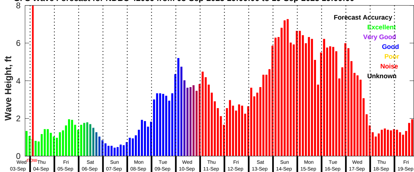
GFS Wave Forecast for NDBC 42036 from 03-Sep-2025 19:00:00 to 19-Sep-2025 19:00:00
