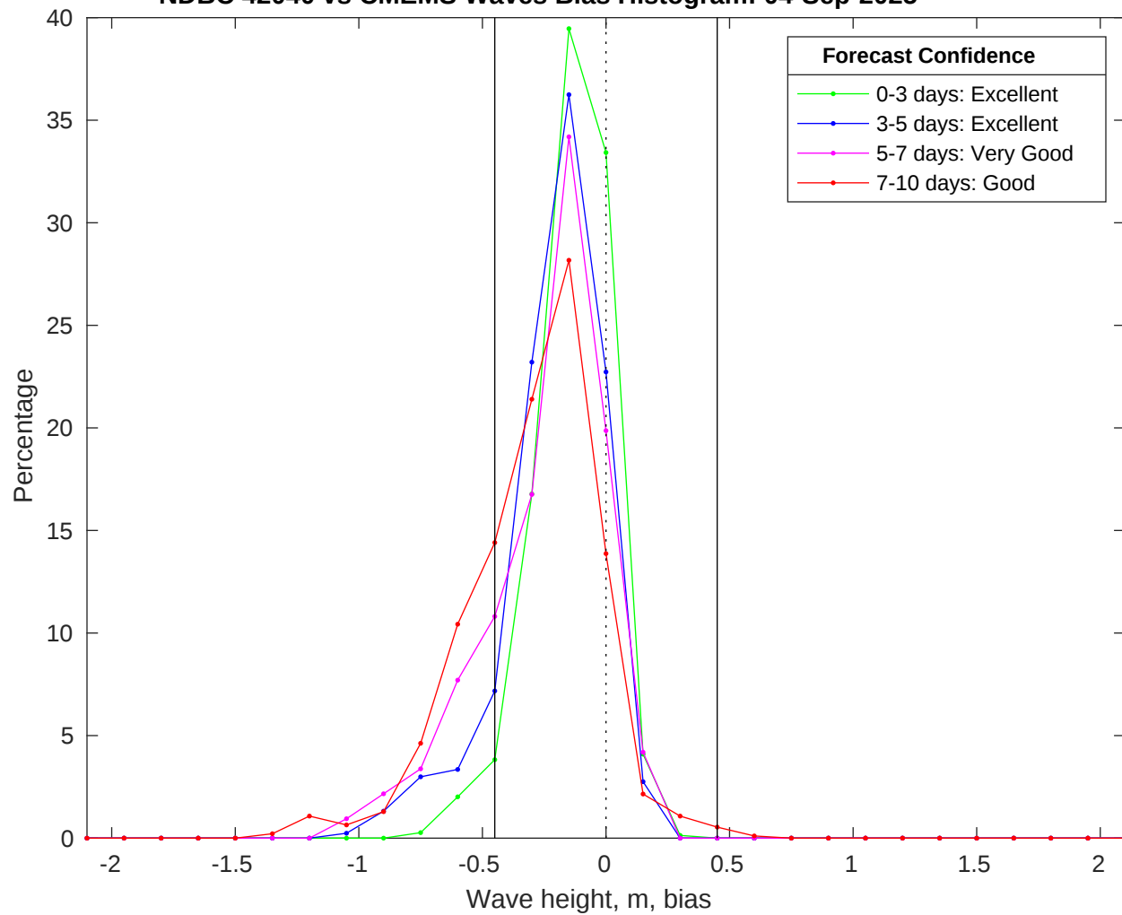
NDBC 42040 vs CMEMS Waves Bias Histogram: 04-Sep-2025
