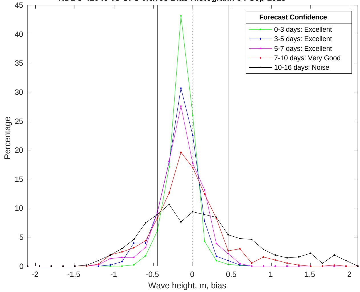
NDBC 42040 vs GFS Waves Bias Histogram: 04-Sep-2025
