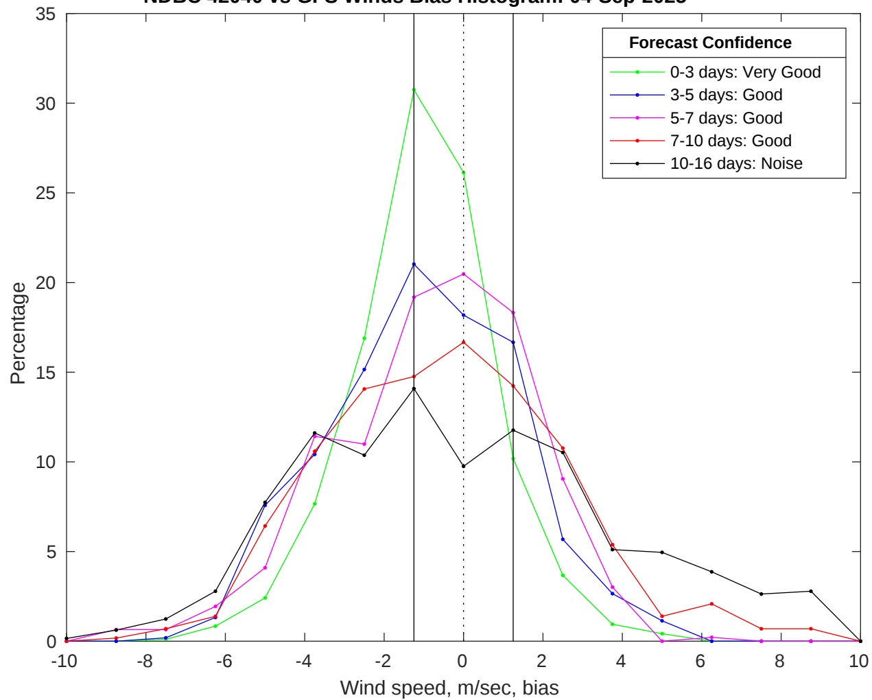
NDBC 42040 vs GFS Winds Bias Histogram: 04-Sep-2025
