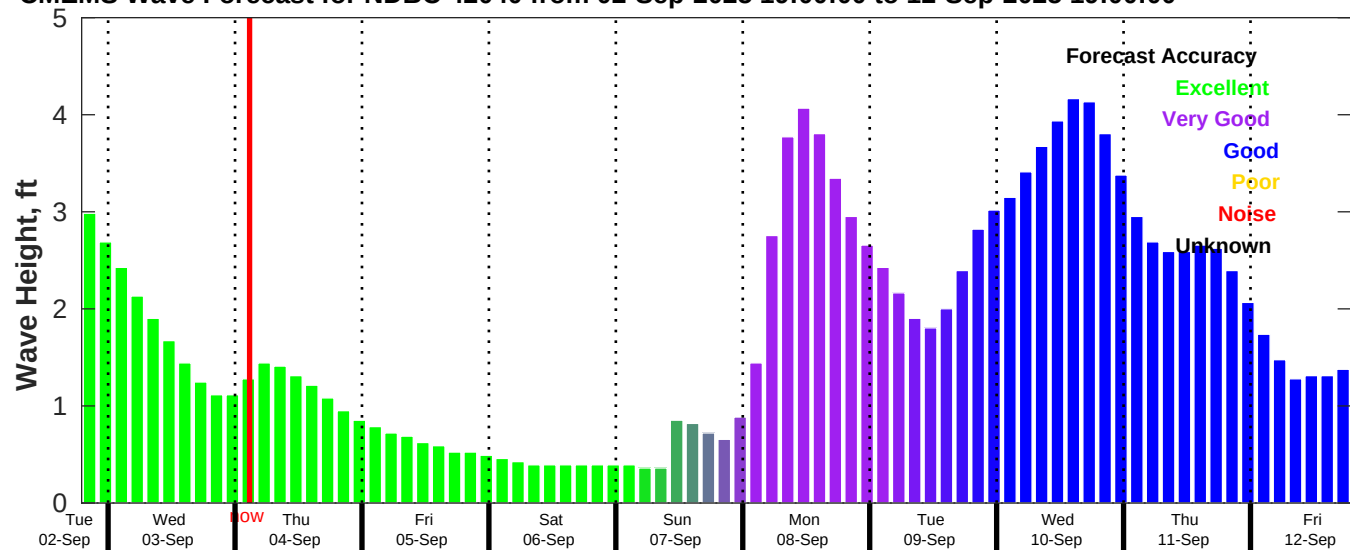
CMEMS Wave Forecast for NDBC 42040 from 02-Sep-2025 19:00:00 to 12-Sep-2025 19:00:00
