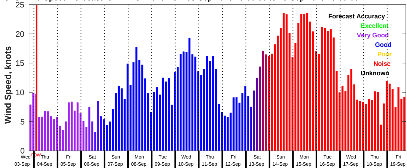
GFS Wind Speed Forecast for NDBC 42040 from 03-Sep-2025 19:00:00 to 19-Sep-2025 19:00:00
