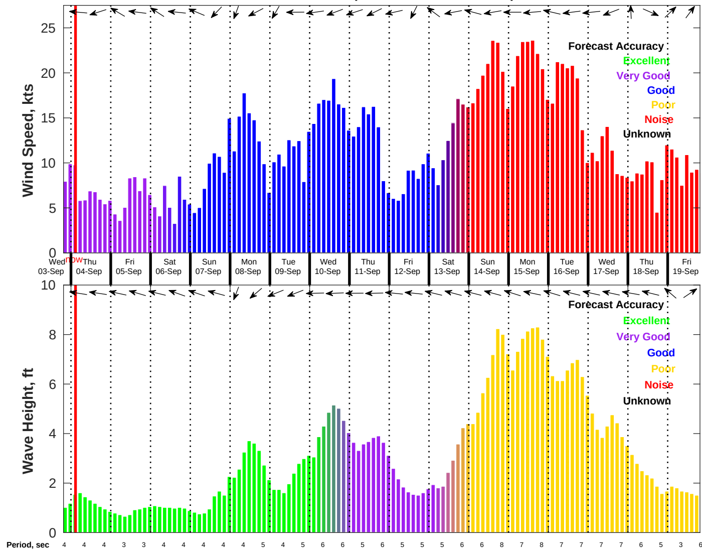
Wind & Wave Forecast for NDBC 42040 from 03-Sep-2025 19:00:00 to 19-Sep-2025 19:00:00
