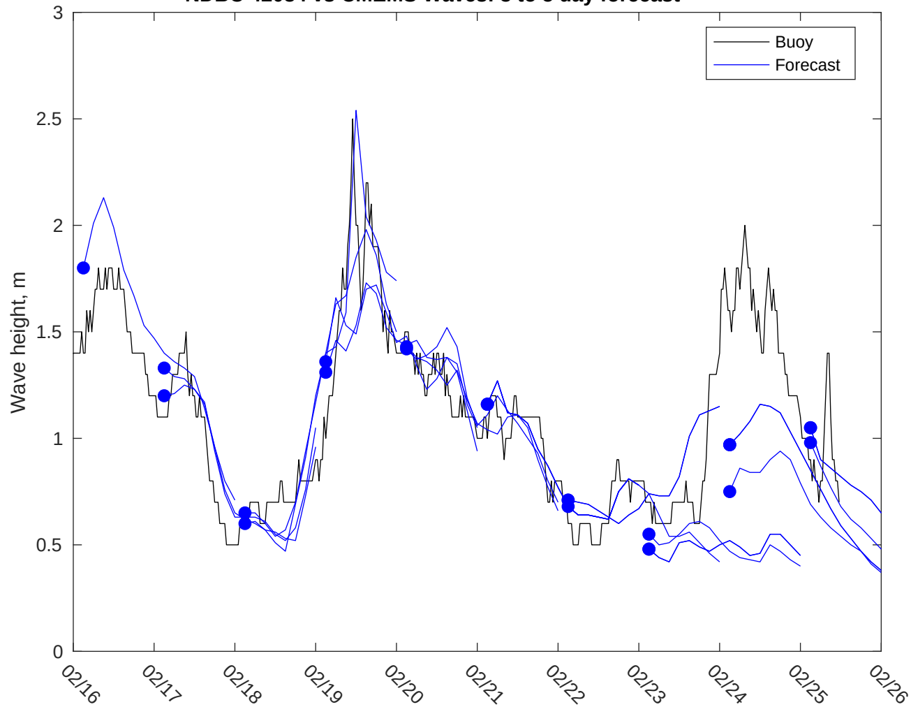
NDBC 42084 vs CMEMS Waves: 3 to 5 day forecast
