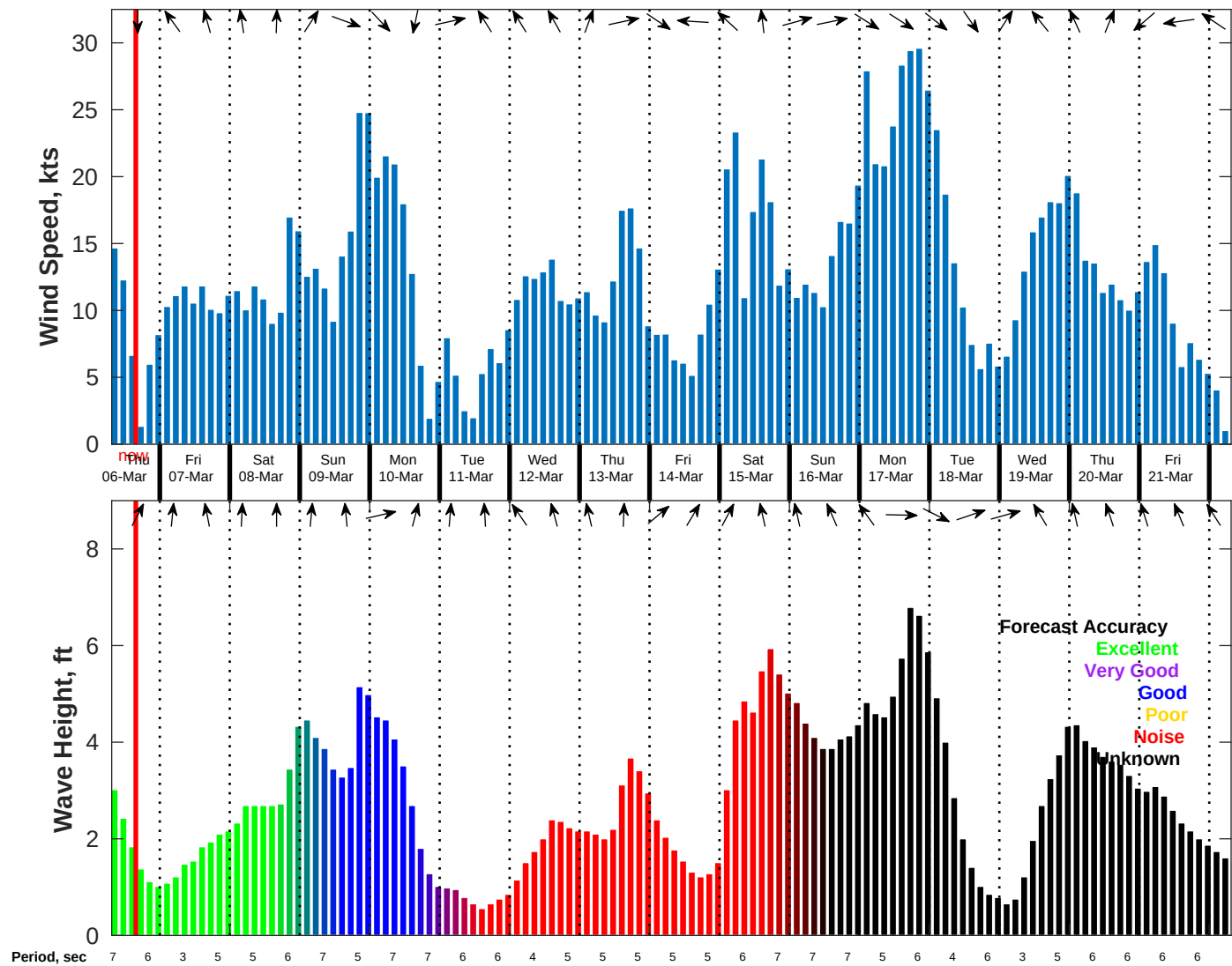
Wind & Wave Forecast for NDBC 42084 from 06-Mar-2025 07:00:00 to 22-Mar-2025 07:00:00
