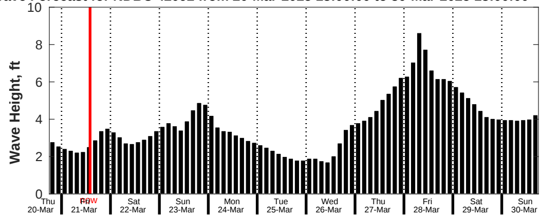
CMEMS Wave Forecast for NDBC 42092 from 20-Mar-2025 18:00:00 to 30-Mar-2025 18:00:00
