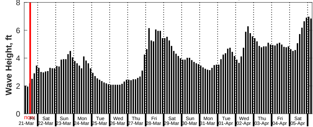
GFS Wave Forecast for NDBC 42092 from 21-Mar-2025 06:00:00 to 06-Apr-2025 06:00:00
