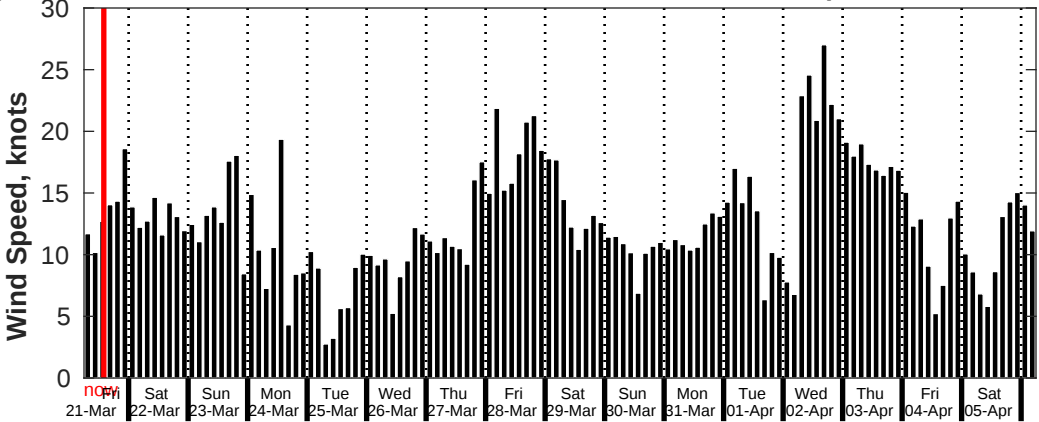
GFS Wind Speed Forecast for NDBC 42092 from 21-Mar-2025 06:00:00 to 06-Apr-2025 06:00:00
