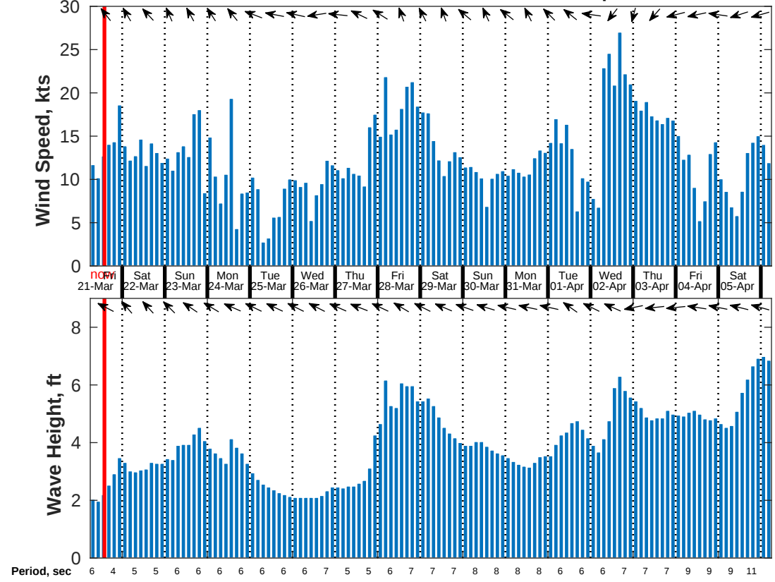
Wind & Wave Forecast for NDBC 42092 from 21-Mar-2025 06:00:00 to 06-Apr-2025 06:00:00
