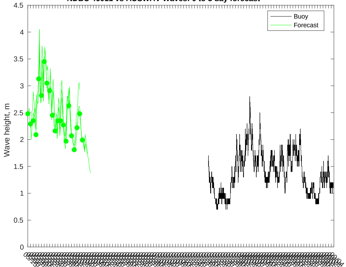
NDBC 46011 vs AUSWAV Waves: 0 to 3 day forecast
