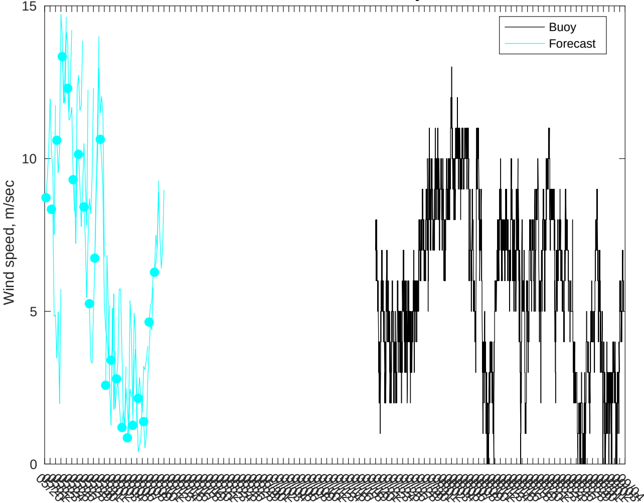
NDBC 46011 vs AUSWAV Winds: 5 to 7 day forecast
