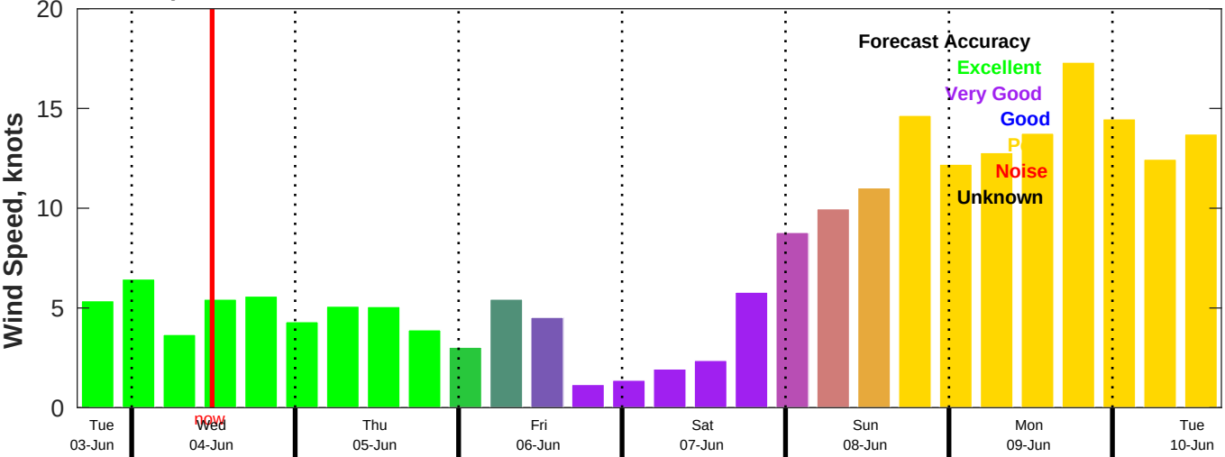
AUSWAV Wind Speed Forecast for NDBC 46011 from 03-Jun-2025 16:00:00 to 10-Jun-2025 16:00:00
