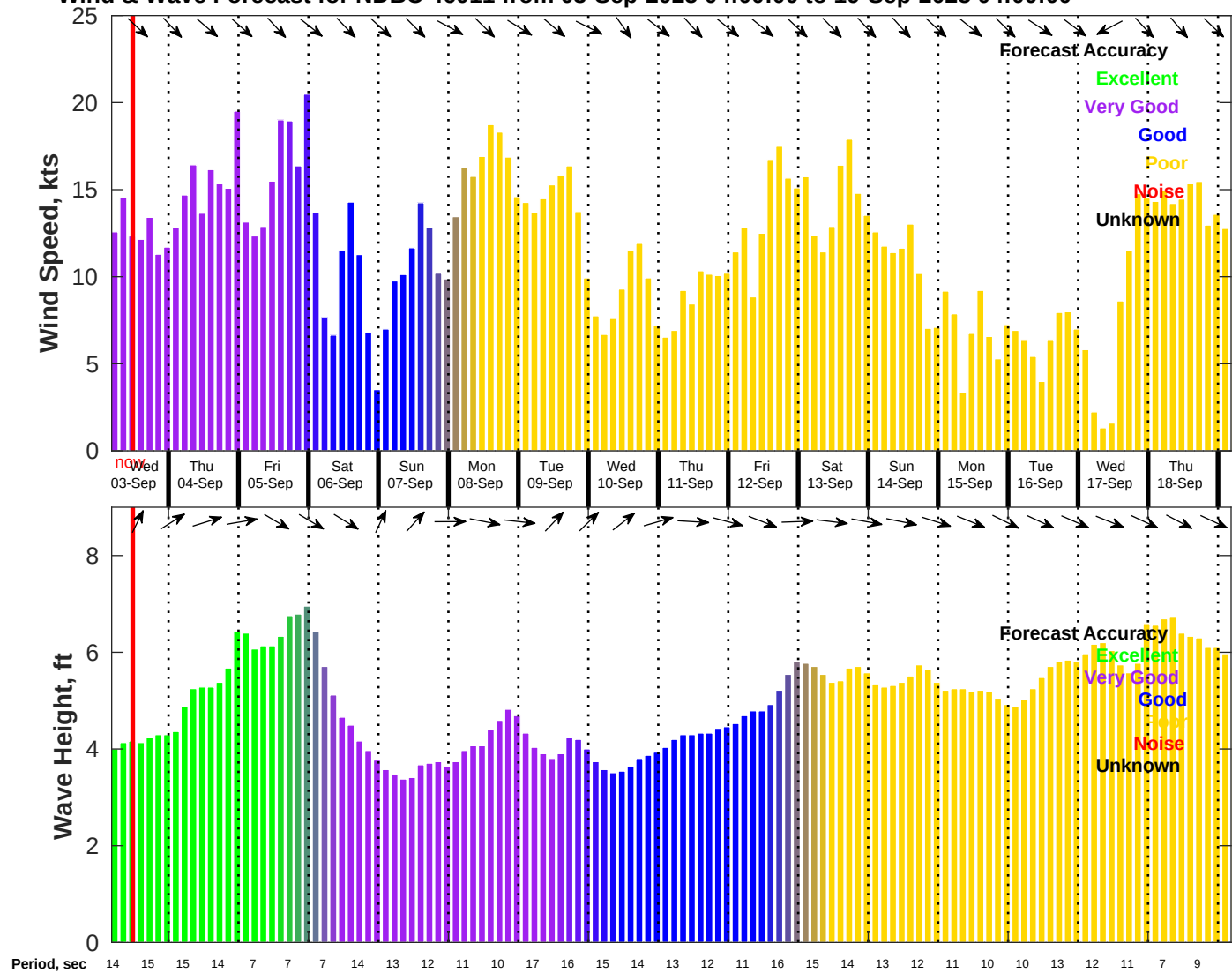
Wind & Wave Forecast for NDBC 46011 from 03-Sep-2025 04:00:00 to 19-Sep-2025 04:00:00
