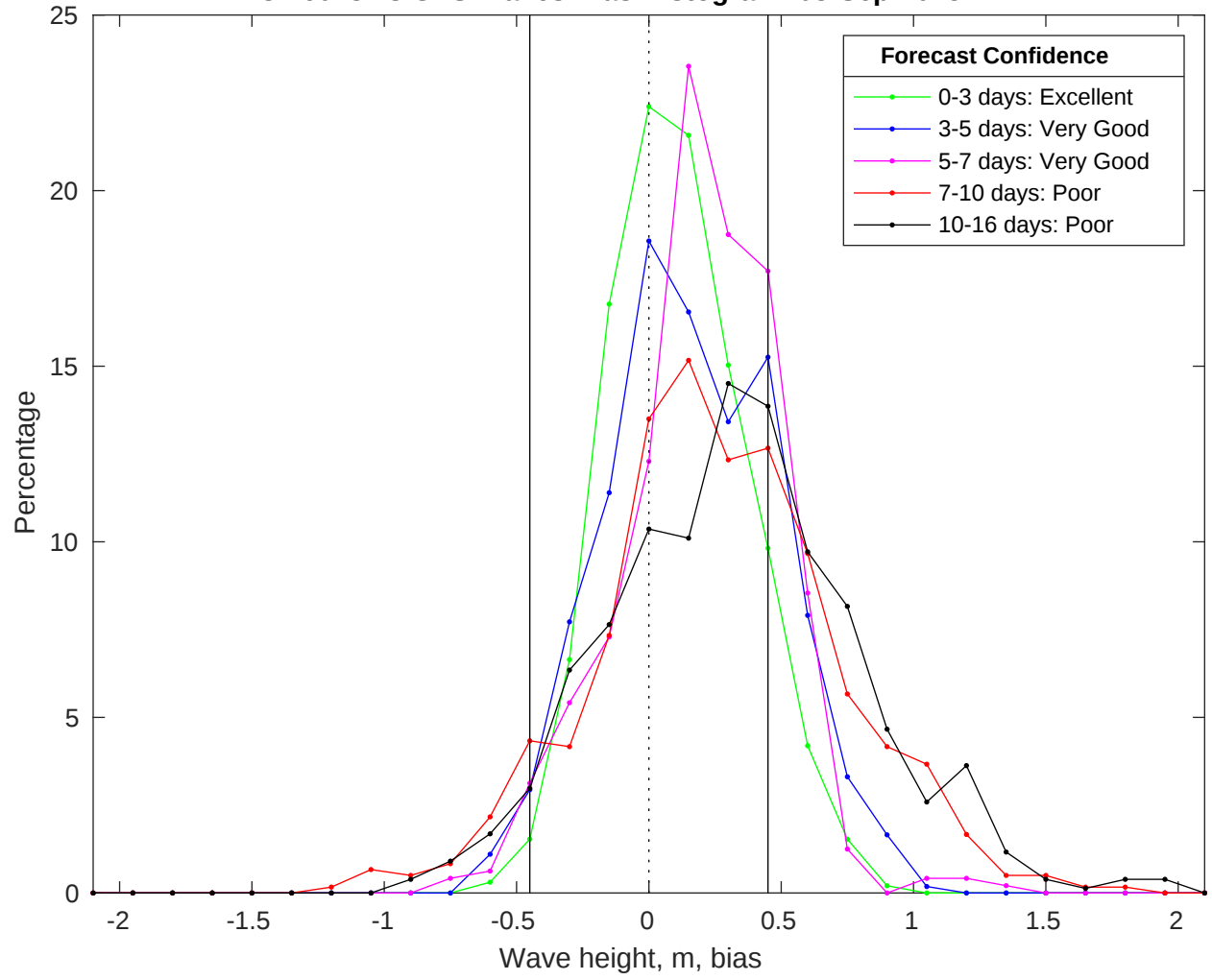
NDBC 46028 vs GFS Waves Bias Histogram: 03-Sep-2025
