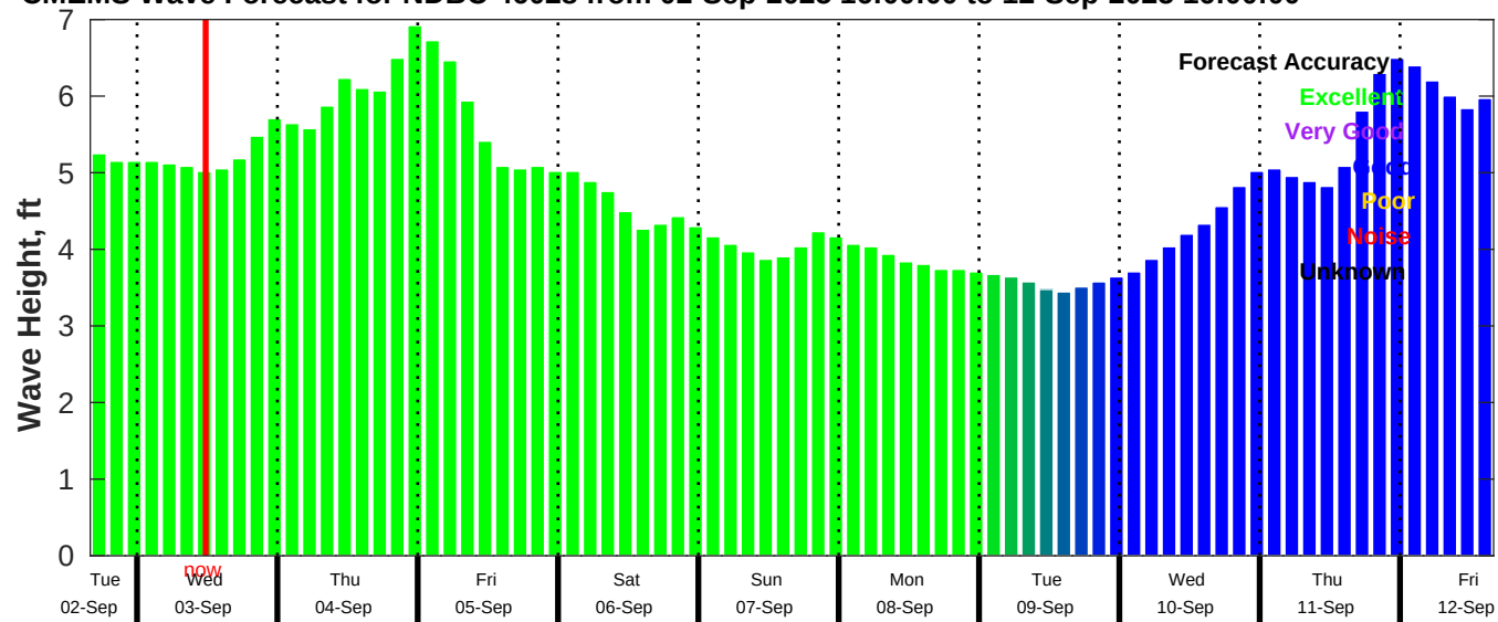
CMEMS Wave Forecast for NDBC 46028 from 02-Sep-2025 16:00:00 to 12-Sep-2025 16:00:00
