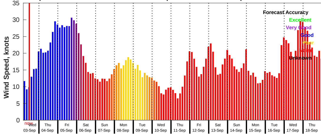
GFS Wind Speed Forecast for NDBC 46028 from 03-Sep-2025 04:00:00 to 19-Sep-2025 04:00:00
