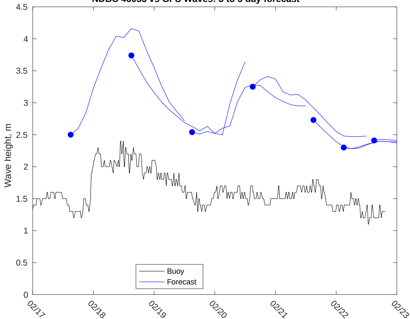
NDBC 46053 vs GFS Waves: 3 to 5 day forecast
