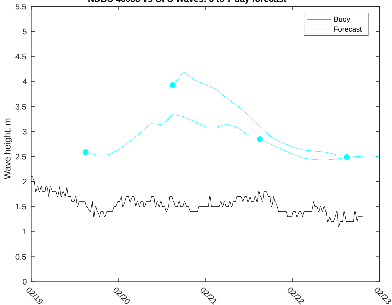
NDBC 46053 vs GFS Waves: 5 to 7 day forecast
