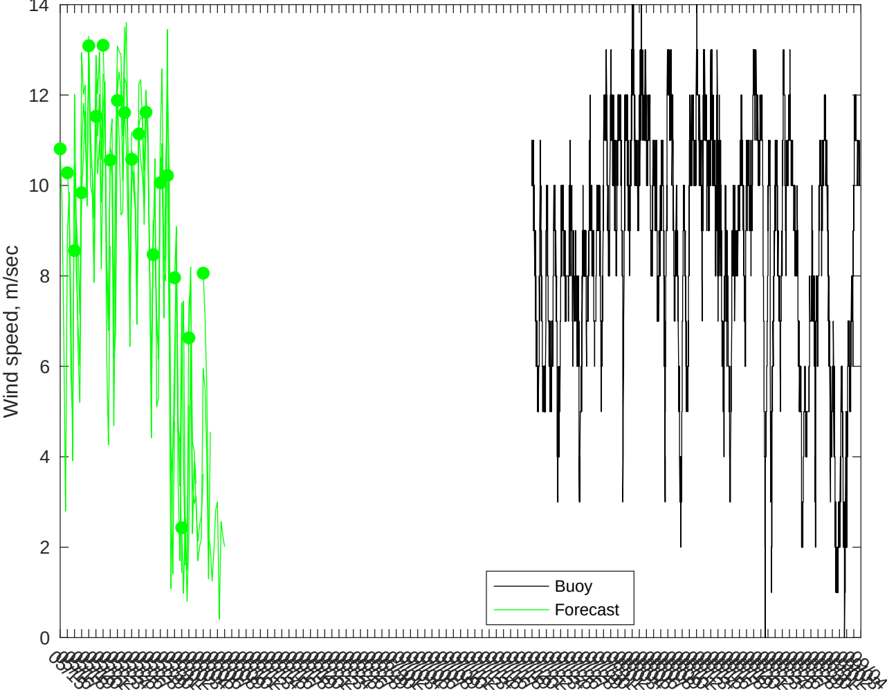
NDBC 46054 vs AUSWAV Winds: 0 to 3 day forecast
