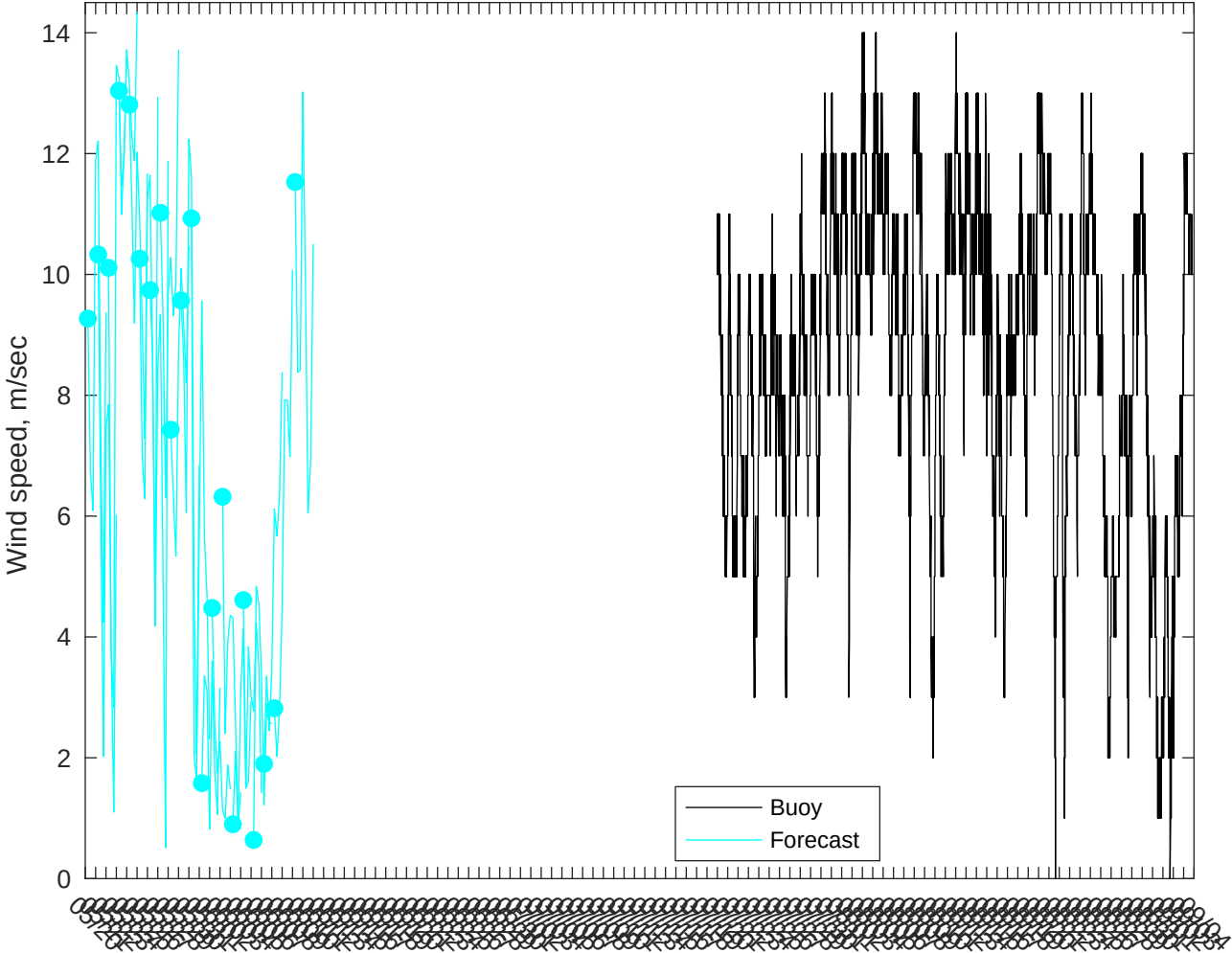
NDBC 46054 vs AUSWAV Winds: 5 to 7 day forecast
