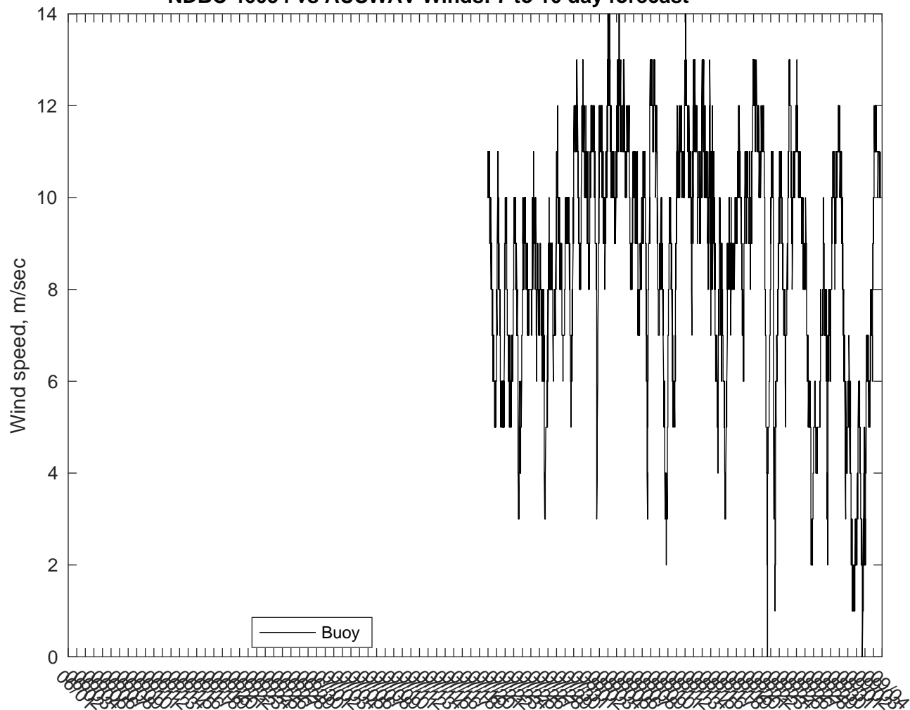
NDBC 46054 vs AUSWAV Winds: 7 to 10 day forecast
