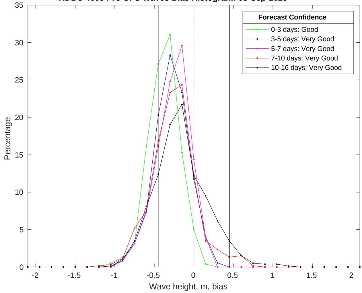
NDBC 46054 vs GFS Waves Bias Histogram: 03-Sep-2025
