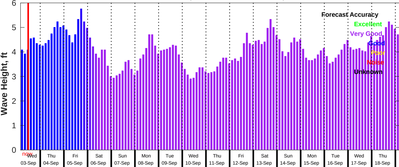
GFS Wave Forecast for NDBC 46054 from 03-Sep-2025 04:00:00 to 19-Sep-2025 04:00:00
