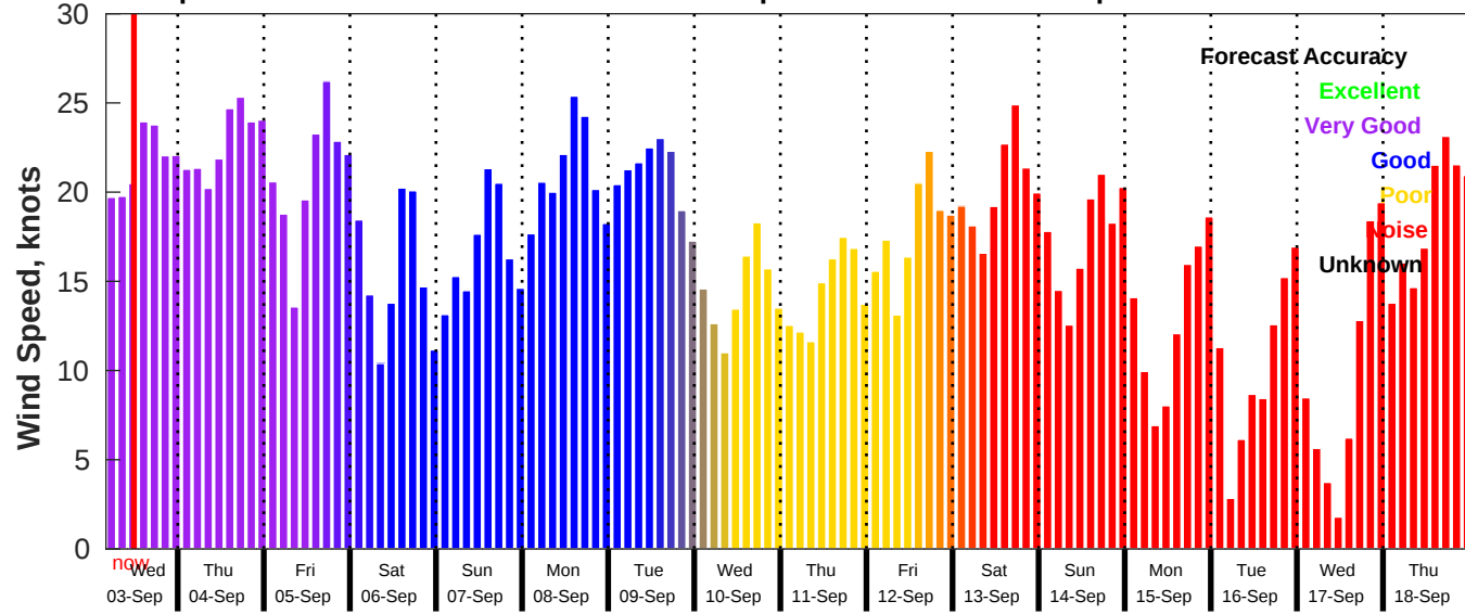
GFS Wind Speed Forecast for NDBC 46054 from 03-Sep-2025 04:00:00 to 19-Sep-2025 04:00:00
