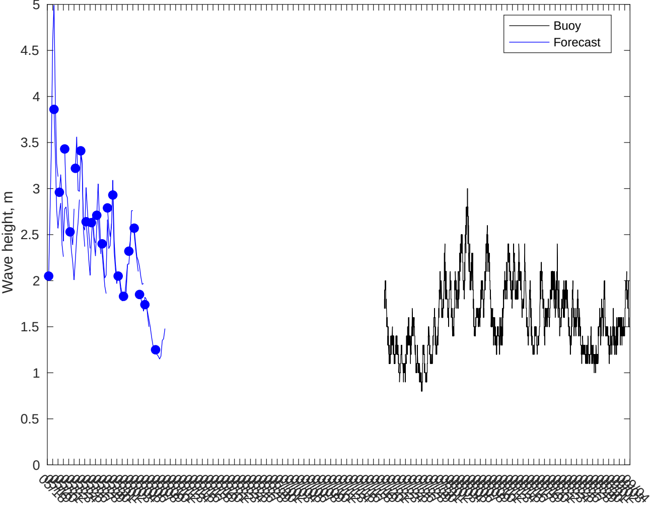
NDBC 46069 vs AUSWAV Waves: 3 to 5 day forecast
