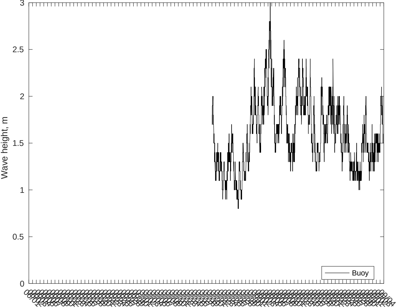
NDBC 46069 vs AUSWAV Waves: 7 to 10 day forecast
