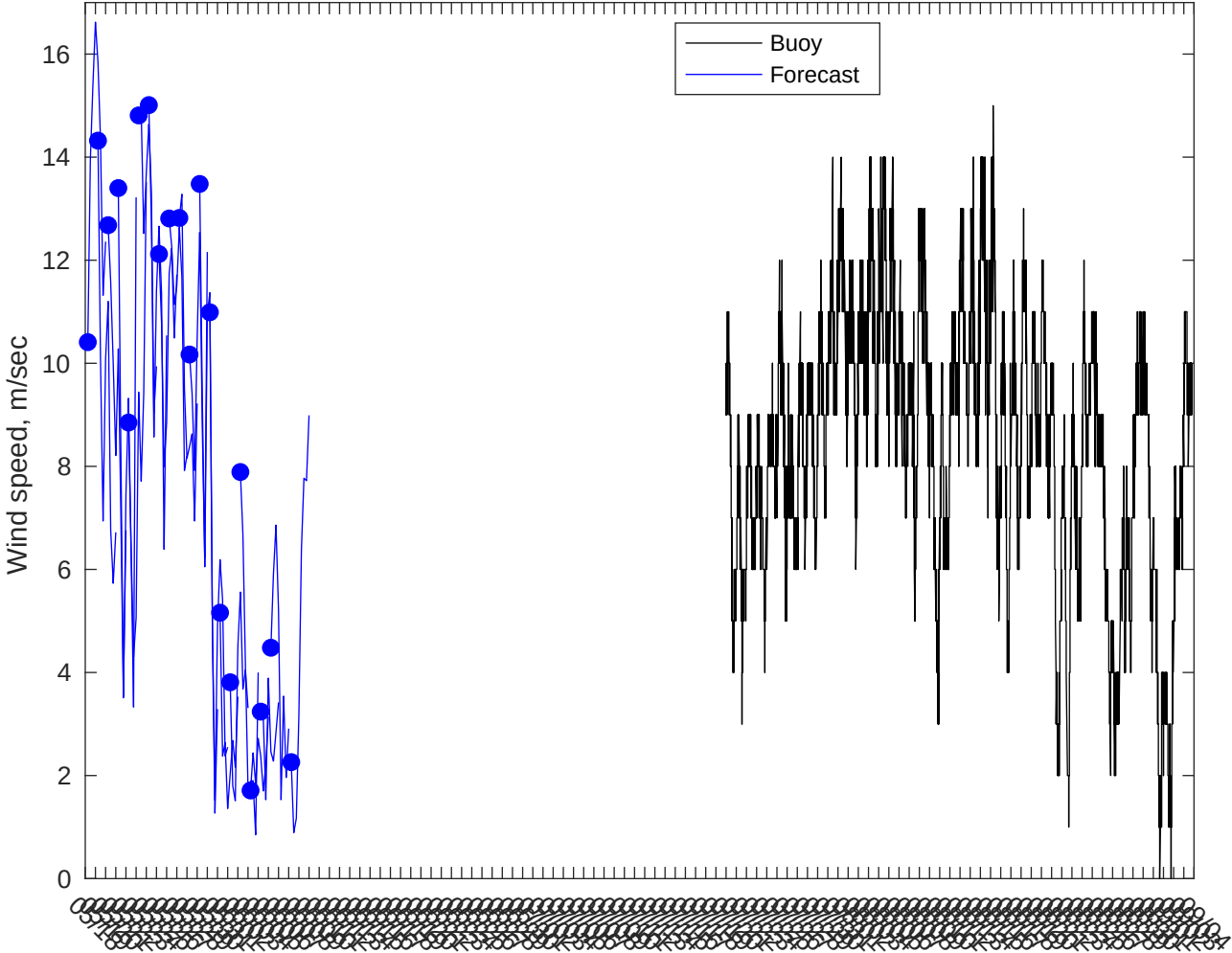
NDBC 46069 vs AUSWAV Winds: 3 to 5 day forecast
