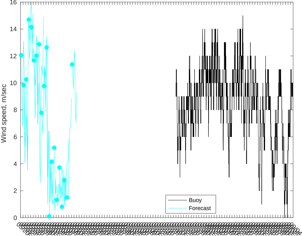
NDBC 46069 vs AUSWAV Winds: 5 to 7 day forecast
