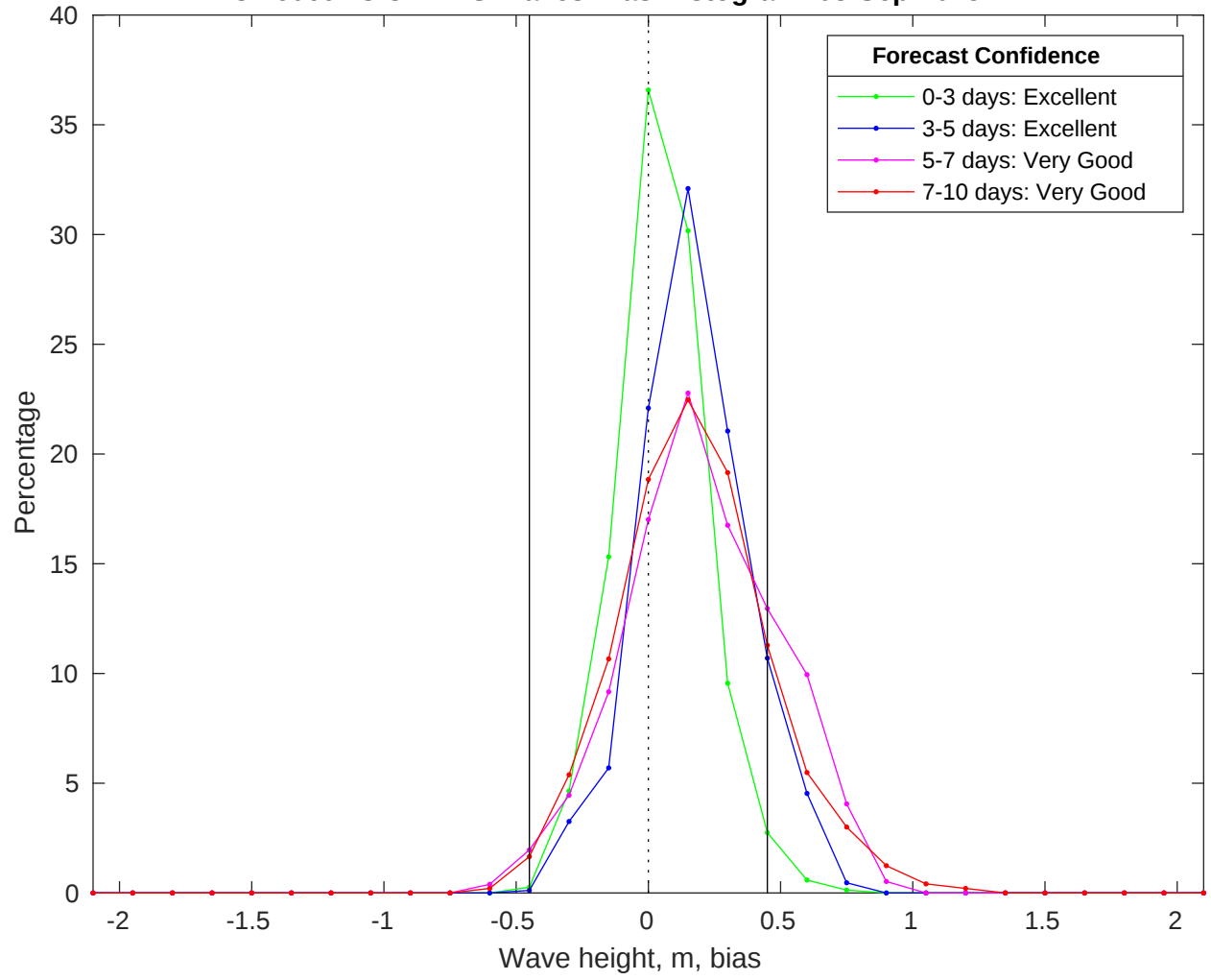
NDBC 46069 vs CMEMS Waves Bias Histogram: 03-Sep-2025
