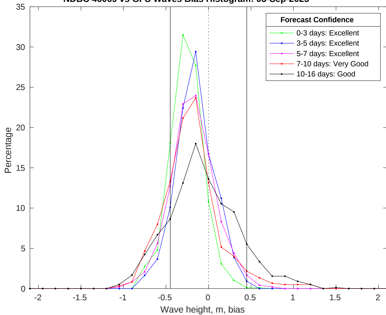
NDBC 46069 vs GFS Waves Bias Histogram: 03-Sep-2025
