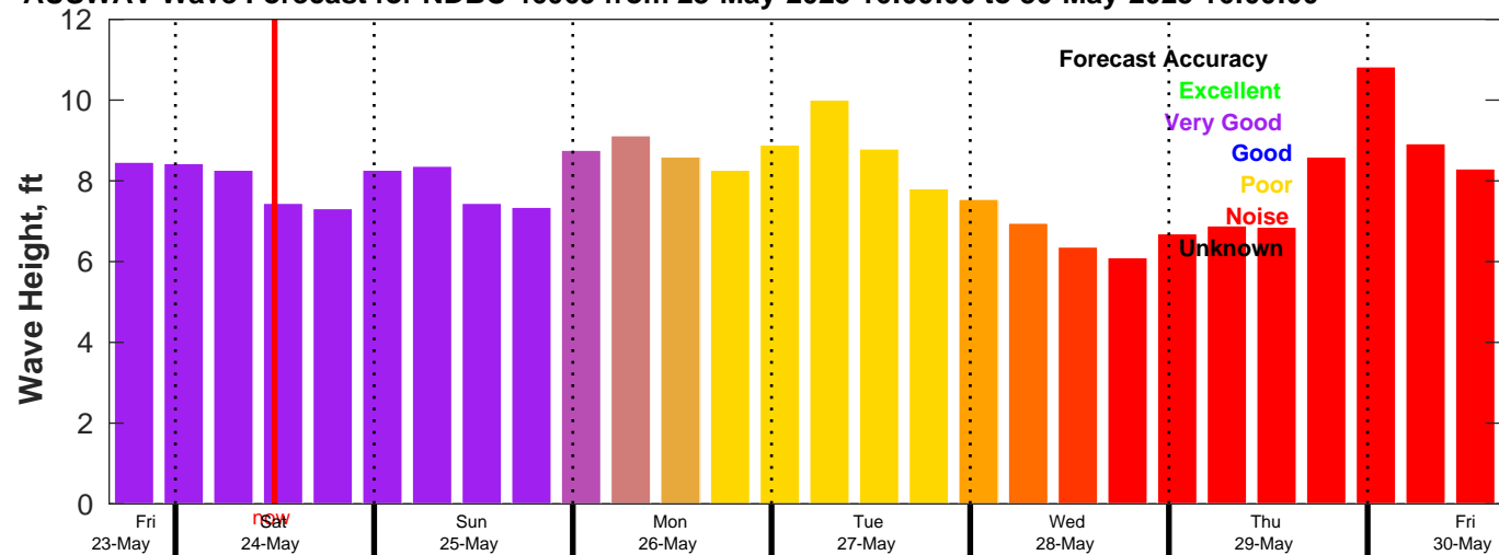
AUSWAV Wave Forecast for NDBC 46069 from 23-May-2025 16:00:00 to 30-May-2025 16:00:00
