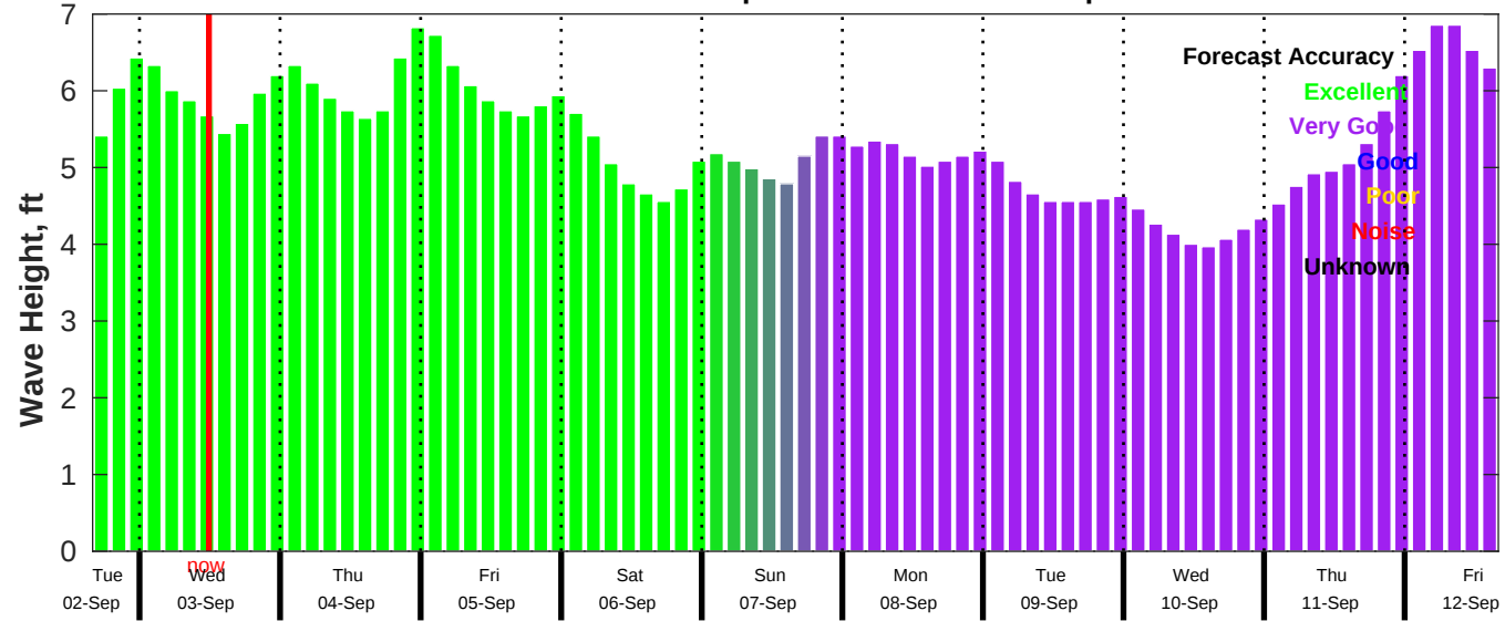
CMEMS Wave Forecast for NDBC 46069 from 02-Sep-2025 16:00:00 to 12-Sep-2025 16:00:00
