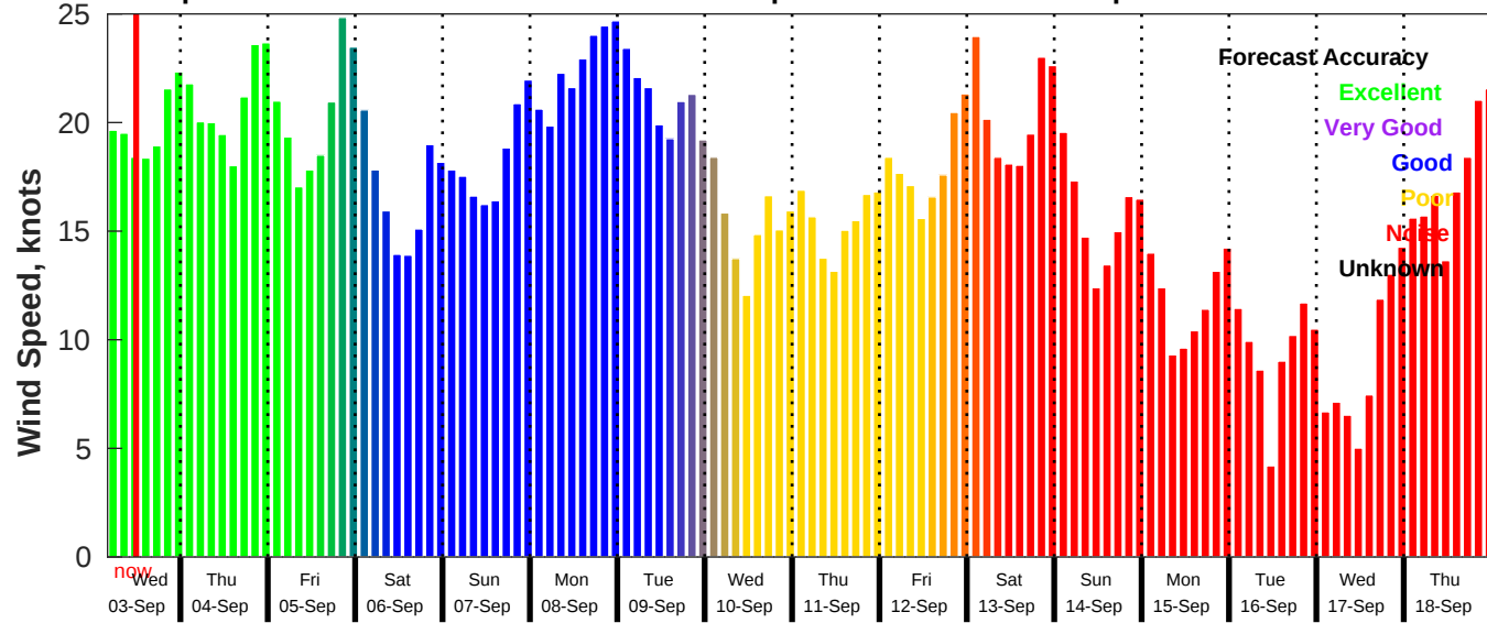
GFS Wind Speed Forecast for NDBC 46069 from 03-Sep-2025 04:00:00 to 19-Sep-2025 04:00:00
