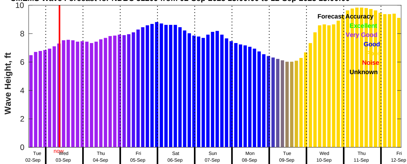
CMEMS Wave Forecast for NDBC 51209 from 02-Sep-2025 13:00:00 to 12-Sep-2025 13:00:00
