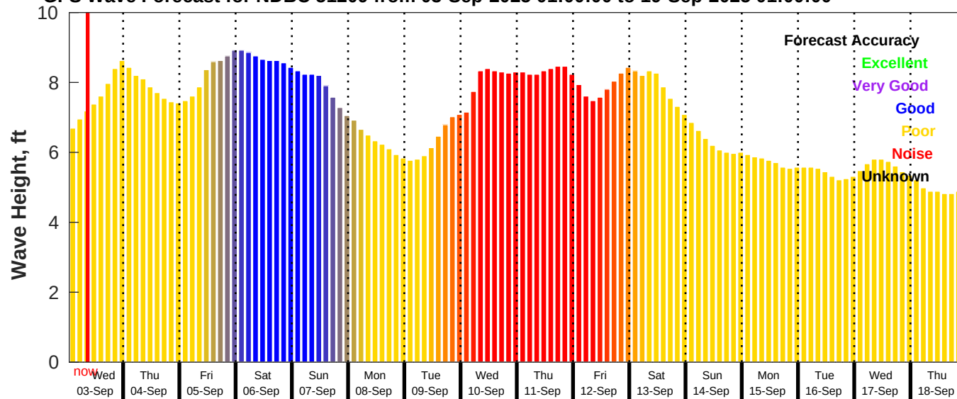
GFS Wave Forecast for NDBC 51209 from 03-Sep-2025 01:00:00 to 19-Sep-2025 01:00:00
