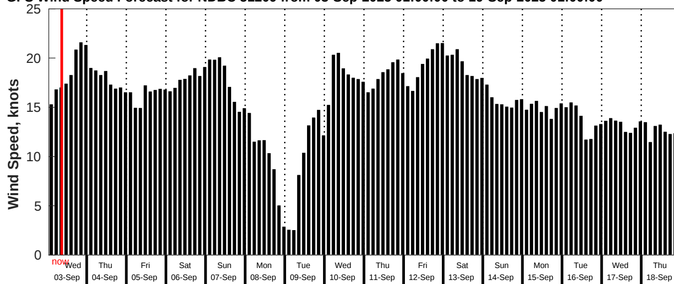
GFS Wind Speed Forecast for NDBC 51209 from 03-Sep-2025 01:00:00 to 19-Sep-2025 01:00:00
