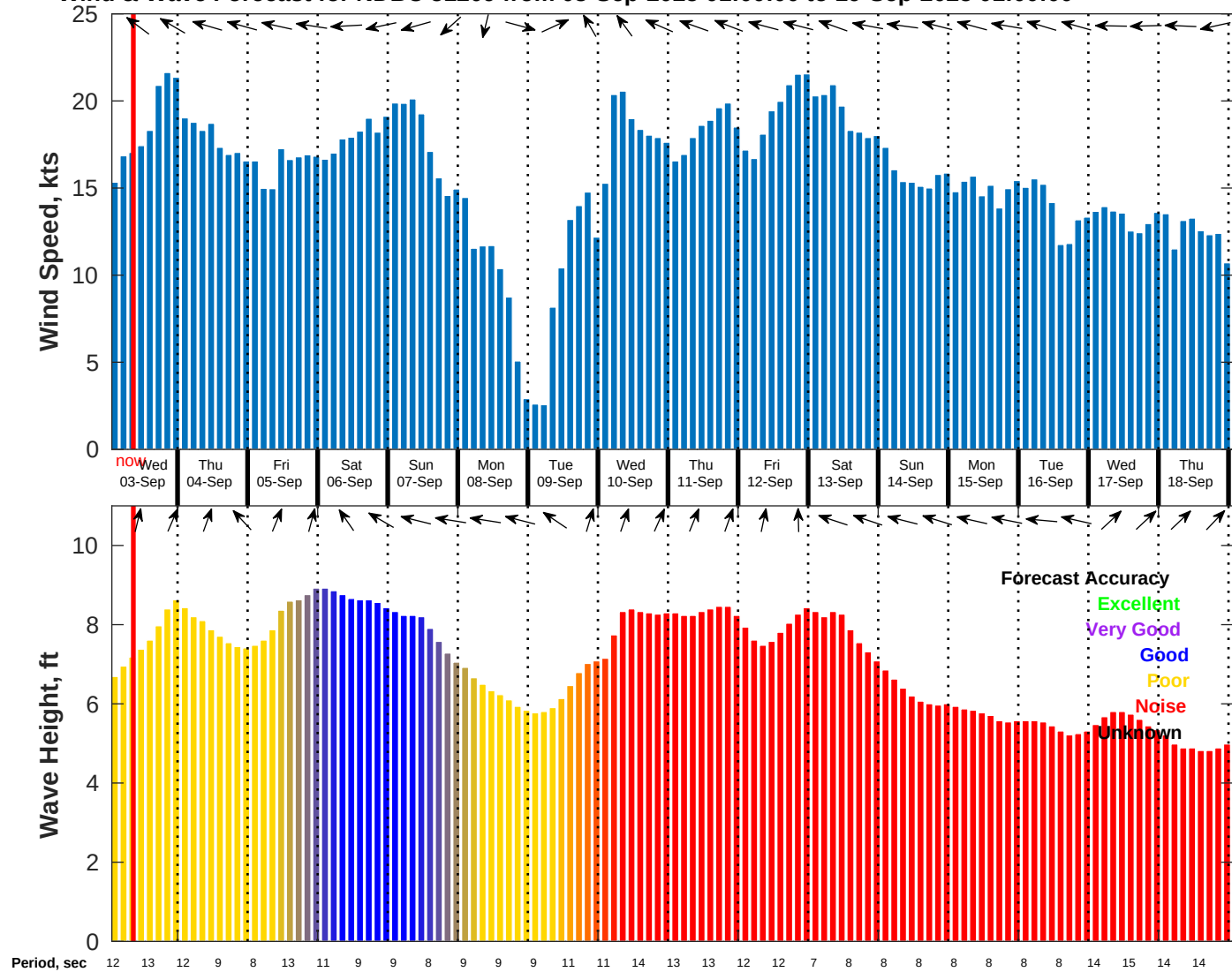
Wind & Wave Forecast for NDBC 51209 from 03-Sep-2025 01:00:00 to 19-Sep-2025 01:00:00
