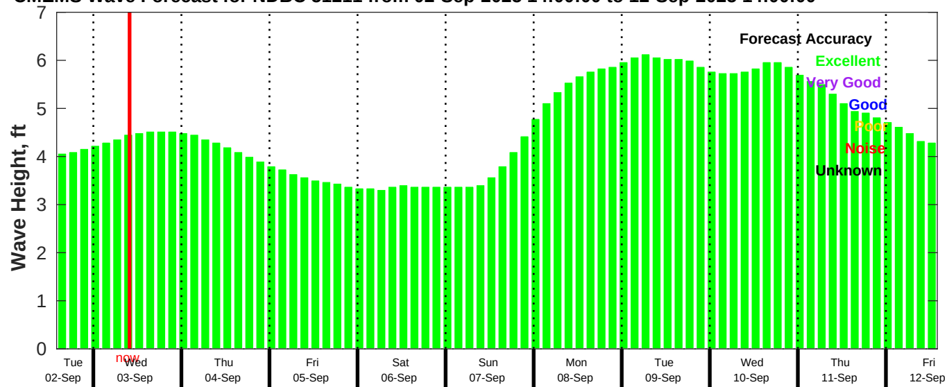
CMEMS Wave Forecast for NDBC 51211 from 02-Sep-2025 14:00:00 to 12-Sep-2025 14:00:00
