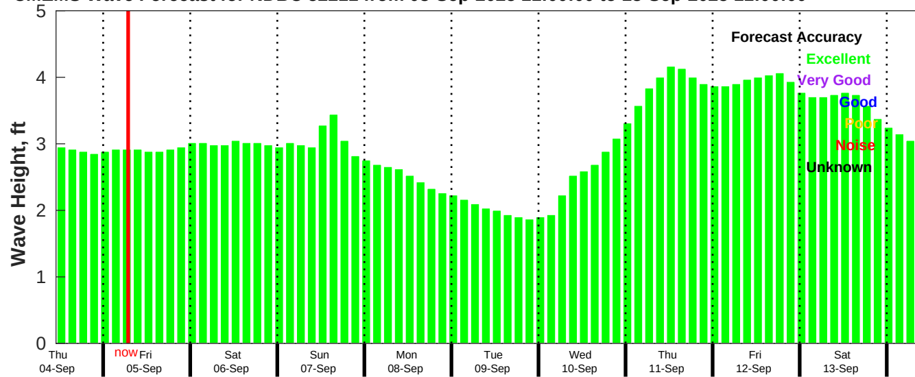
CMEMS Wave Forecast for NDBC 52211 from 03-Sep-2025 11:00:00 to 13-Sep-2025 11:00:00
