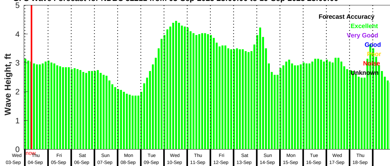
GFS Wave Forecast for NDBC 52211 from 03-Sep-2025 23:00:00 to 19-Sep-2025 23:00:00
