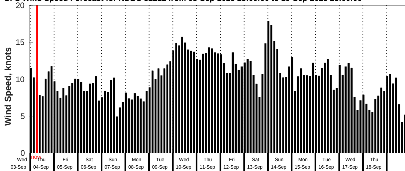
GFS Wind Speed Forecast for NDBC 52211 from 03-Sep-2025 23:00:00 to 19-Sep-2025 23:00:00
